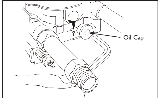
Figure 17 - Changing Pump Oil
